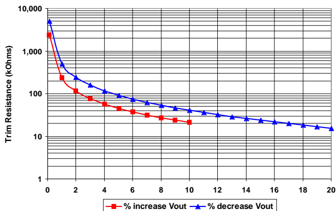
Figure C: Trim Graph for 1.8Vout module
